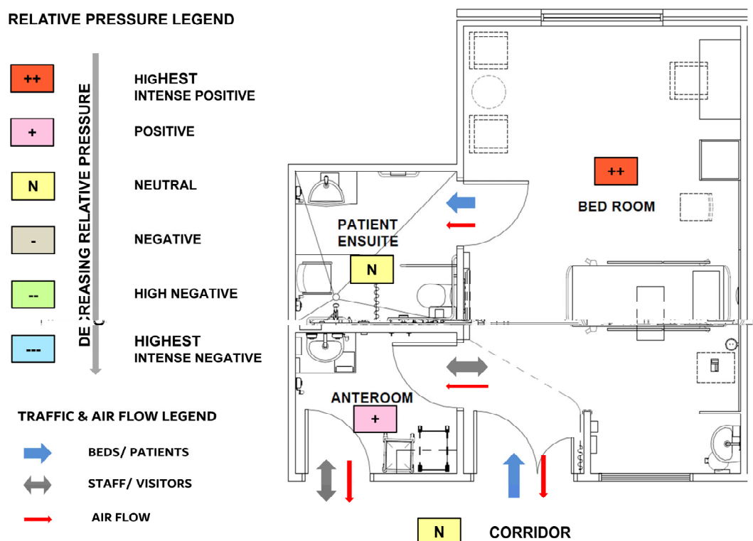
Figure 19: Typical Positive Pressure Isolation Room with Anteroom & Ensuite, showing airflows and relative pressure gradients
